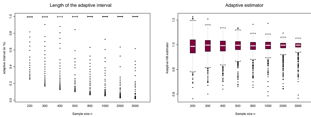
Figure 6. Box-plots of selected intervals (in %) and the adaptive estimators for Pareto d.f. from 500 realization for different sample sizes.
